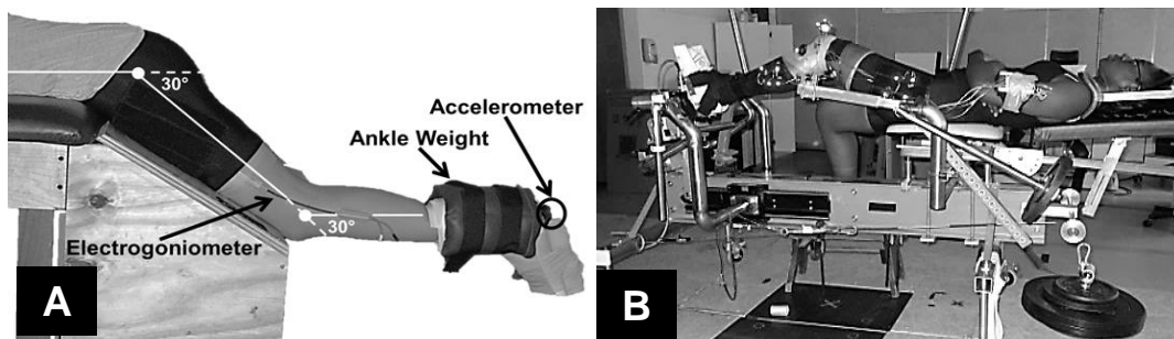
Figure 1. A) Participant positioning during hamstring musculo-articular stiffness ( K_{HAM} ) assessments. B) The Vermont Knee Laxity Device (VKLD).
