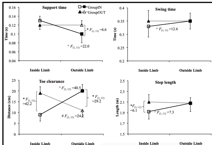
Figure 2: Overall step kinematic variables that displayed a significant limb-type \times limb-side interaction. Open symbol indicates prosthetic limb, whereas solid black symbol indicates non-prosthetic limb. * indicates a significant difference between prosthetic limb-side groups (GroupIN, GroupOUT) for a given limb side. Significant inter-limb differences within a group: # = for GroupOUT, ^ = GroupIN. All comparisons: p < .05 .
