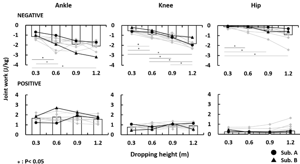
Figure 2: Joint work at each drop height.
