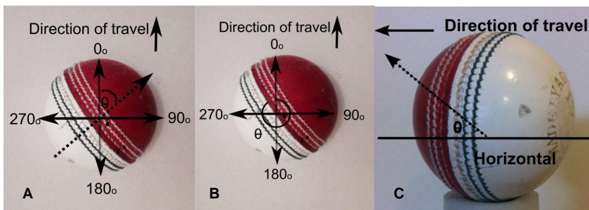
Figure 1a. A superior view of the spin axis azimuth angle, whereby ( \theta_{\vec{\omega}} ) is the angle measured between the angular velocity vector (dotted line) and the x -axis of the global.
