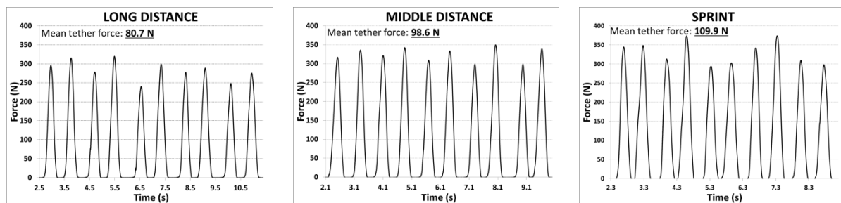
Figure 1: A measured force–time curve for one swimmer (and mean tether force) during 10 arm strokes, at the three paces of swimming.
