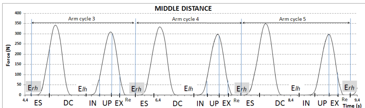
Figure 2: example of kinematic-dynamic coupled measurements. The curve represents a force signal measured for a swimmer during 3 right arms cycles (3rd, 4th and 5th). Erh defines the entry of the right hand in the water; Elh : the entry of the left hand. ES : entry and stretch phase; DC : downsweep to catch; IN : insweep; UP : upsweep; EX : exit; Re : recovery of the arm.
