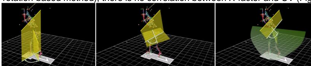
Figure 2: various X-factor computation methods
